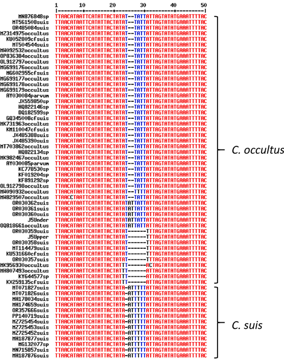
Fig. 1. A 50-bp excerpt of a multiple sequence alignment of Cryptosporidium ssu rDNA reference sequences in the NCBI Database (indicated by GenBank accession numbers and the epithet originally provided for each sequence ('cf. suis ', ' occultus ', ' parvum ', 'sp.', or ' suis '). The species names to the right of the brackets are those that we would consider applicable to the respective sequences.
