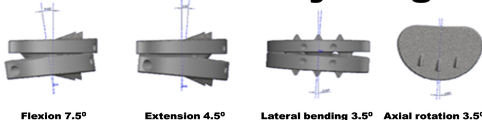
Fig. 2. Drawing and dimensions of the ADDISC complete lumbar disc prosthesis (measurements are in millimeters and angles in degrees). We also show its mobility ranges in each axis.
