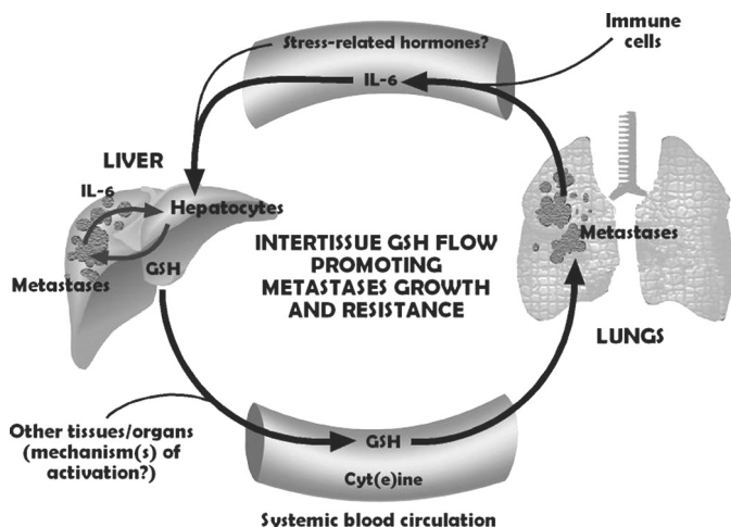
FIGURE 6. The IL-6/GSH interorgan cycle: a tumor growth-promoting mechanism. The liver is the major source of GSH released to the bloodstream. Tumor-derived IL-6 (and perhaps, under stress conditions, other signals, such as different stress-related hormones (1)) acts as a GSH release activator. Tumor GGT activity degrades plasma GSH, providing extra Cys for tumor GSH synthesis (12). Whether other tumor-derived signals activate hepatic GSH release in hosts bearing other cancer types and how each specific tissue microenvironment may influence this systemic flow are open questions.
