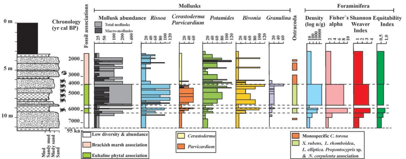
Figure 4. Downcore plots of total mollusk content, abundance of Bivonia , Cerastoderma , Parvicardium , Rissoa , Granulina and Potamides representatives, ostracoda associations, and the Density index, Shannon-Weaver index, Fisher's alpha index, and Equitability index of foraminifera, together with the environmental interpretation.
